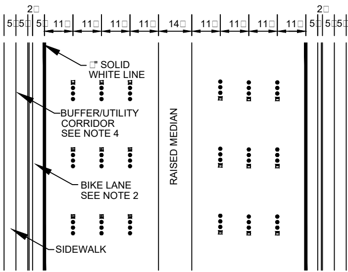
130 FT. STREET
