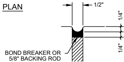
SEALANT DETAIL
