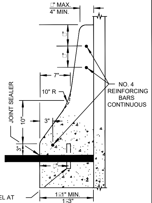
TYPE B
