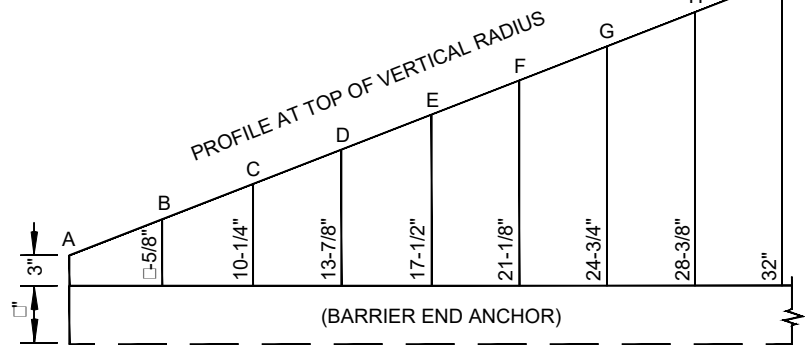
TRANSITION OF END OF BARRIER
