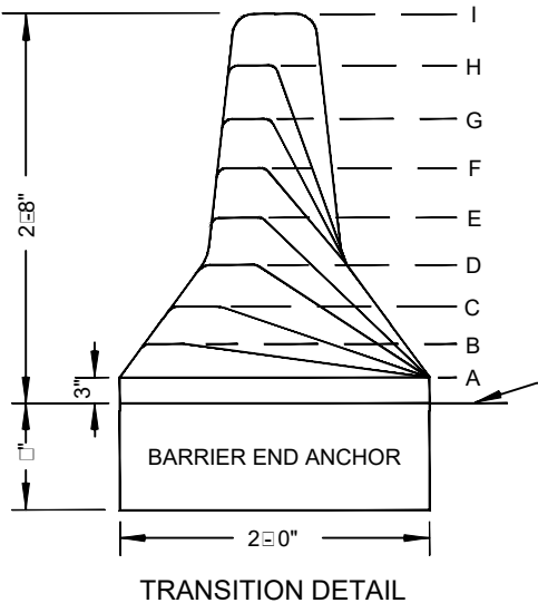
TRANSITION DETAIL
