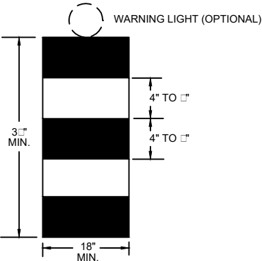
TRAFFIC DRUM
