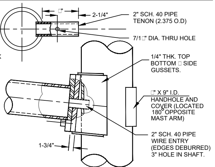
POLE MOUNTING DETAIL
