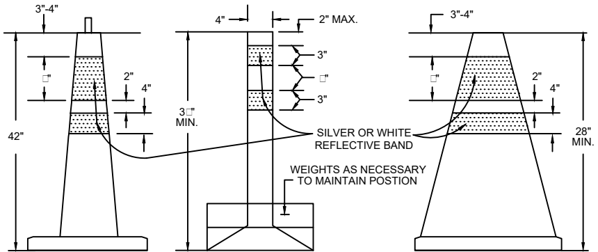
TRAFFIC CONES
