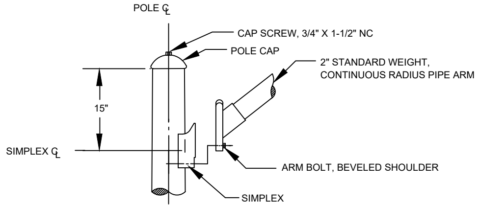
PIPE ARM
