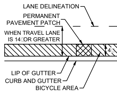
ROADWAY WITH SHARED BICYCLE/VEHICLE LANE
