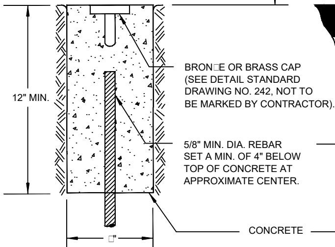
SECTION A-A TYPE II-A UNPAVED STREET
