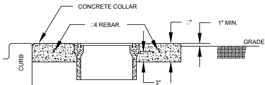
TYPICAL SECTION
