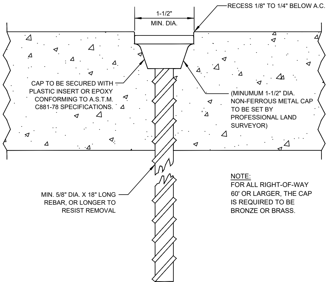
TYPE III MONUMENT
