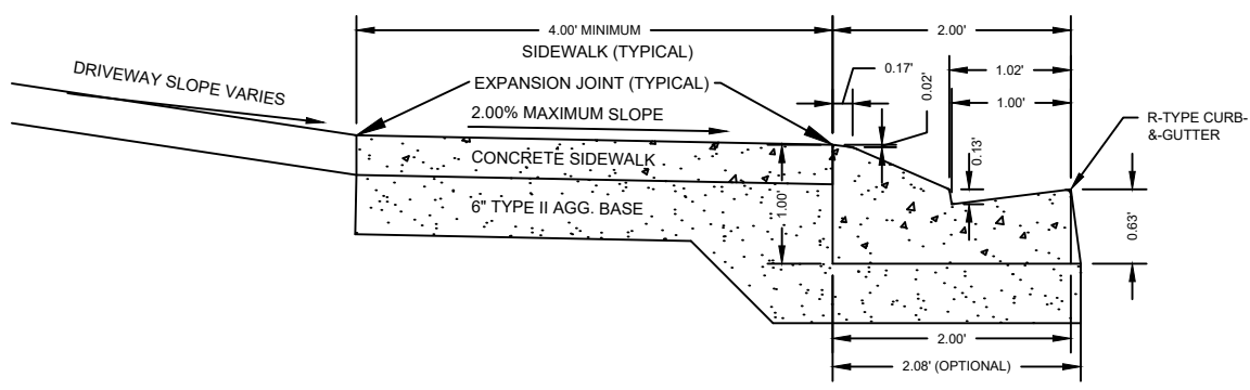
SECTION B-B
